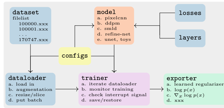
Figure 5.1: The loss and layer functions are used to create models. The trainer is fed by the dataloader and trains the model on multiple GPUs. The exporter is used to customize trained models for deployment. We use these python libraries to implement spreco: 1) tensorflow; 2) numpy; 3) pyyaml; 4)matplotlib; 5)scikit-image; 6) tqdm.
