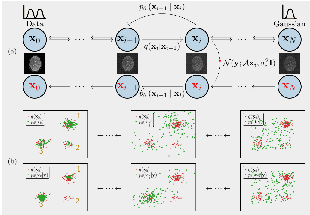
Figure 3.1: Overview of the proposed method. (a) The unknown data distribution q(\mathbf{x}_0) of the training images goes through repeated Gaussian diffusion and finally reaches a known Gaussian distribution q(\mathbf{x}_N) , and this process is reversed by learned transition kernels p_\theta(\mathbf{x}_{i-1} | \mathbf{x}_i) . To compute the posterior of the image p(\mathbf{x} | \mathbf{y}) , a new Markov chain \tilde{p}_\theta(\mathbf{x}_{i-1} | \mathbf{x}_i) is constructed by incorporating the measurement model into the reverse process (red chain). (b) Training samples (red dots) from a mixture of bivariate Gaussian distribution are shown. The upper and bottom rows illustrate how samples (green dots) gradually gather around training samples in the reverse process, without and with the observation, respectively. In this example, the likelihood for the observation was a bivariate Gaussian mixture, so that cluster 2 has a lower and cluster 3 has a higher probability.
