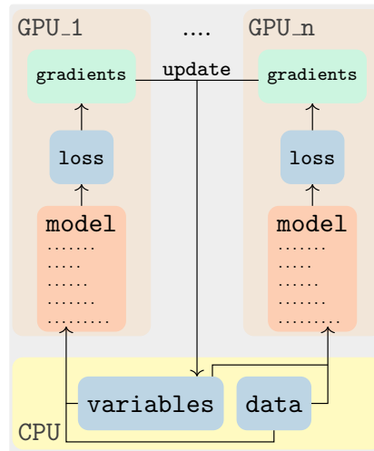
Figure 5.2: Data parallel training. The trainable variables are shared across GPUs and dataloader feeds data to every GPU worker.
